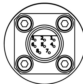
Glenair 5506-1508 Connector Pinout
